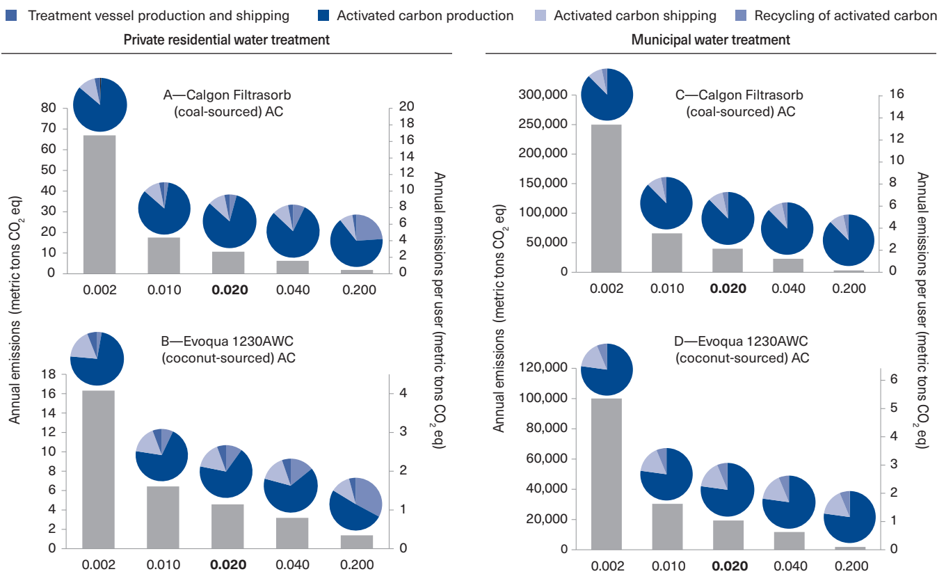
FIGURE 1: Total Greenhouse Gas Emissions (Bar Charts) and Components (Pie Charts)
