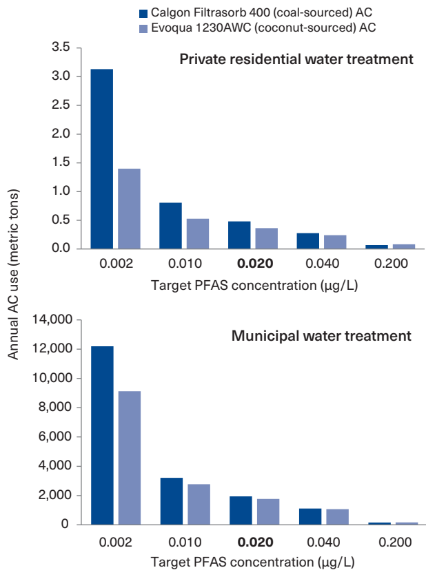
FIGURE 2: Estimated Annual Activated Carbon Use for Coal vs Coconut Source
