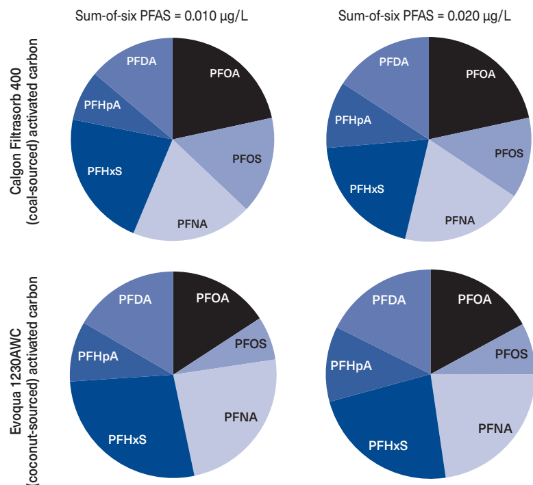
FIGURE 3: Estimated Activated Carbon Usage for Individual PFAS in Municipal Water Treatment Scenarios
